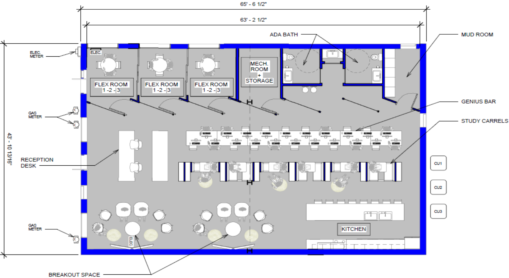
1 APPROXIMATE EXISTING FLOOR PLAN W/ DEMO A100 1/8" = 1' - 0"
