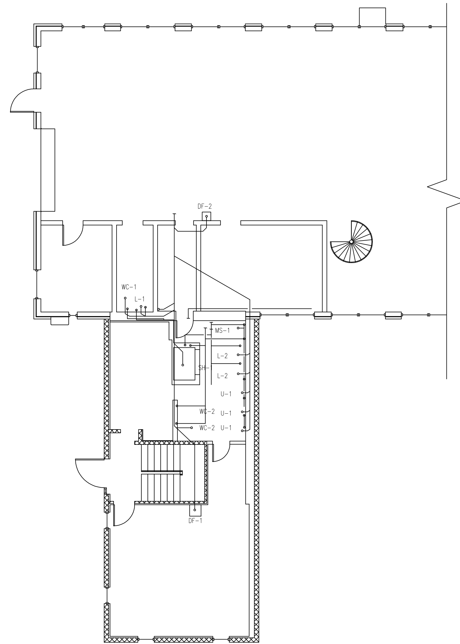
FIRST FLOOR PLUMBING PART PLAN A
